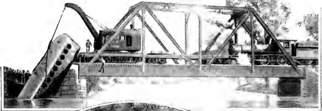
Above, the crane has its "hands full," but fortunately for it the car is of steel and can stand the heaviest pull
